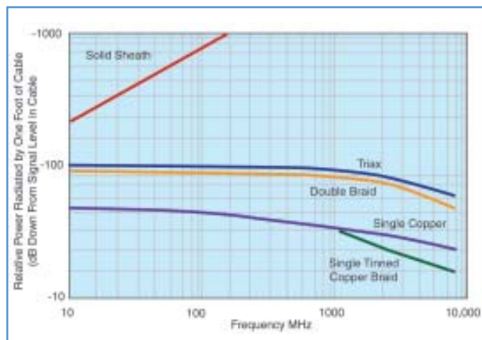
Fig. 9 Shielding Effectiveness
