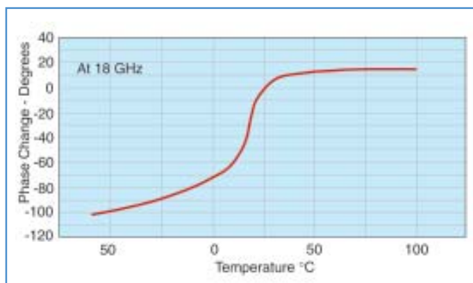
Fig. 10 Phase Stability
