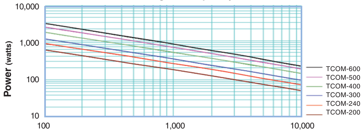
Power Handling vs. Frequency (Maximum)
