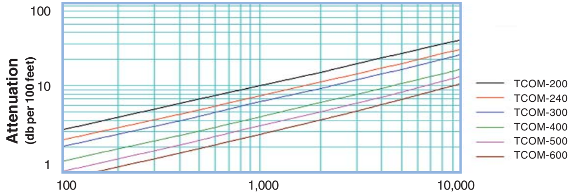
Attenuation vs. Frequency (Typical)
