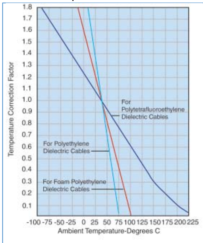
Fig. 6 Power Temperature Correction Factor
